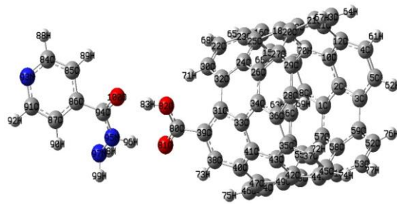
(f-SWCNT/Isoniazid ۹)
